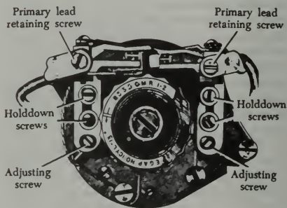
FIGURE 4-37. Magneto breaker points and compensated cam.
